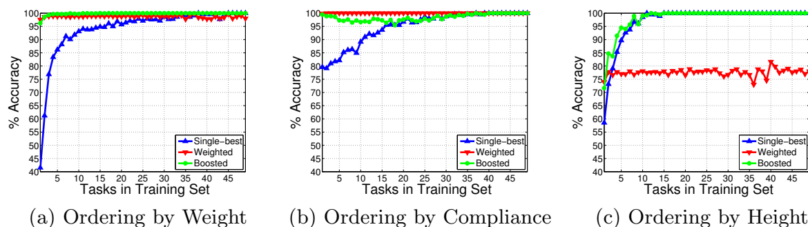
Figure 5.6: The average accuracy as the number of tasks used for training is increased. The blue line is the accuracy achieved when picking just the single-best context; the red line is the accuracy achieved when the contexts are weighted in proportion to their individual accuracies; and the green line is the accuracy achieved when using boosting. The results are averaged over 50 sets of training tasks for each size from 1 to 49.
